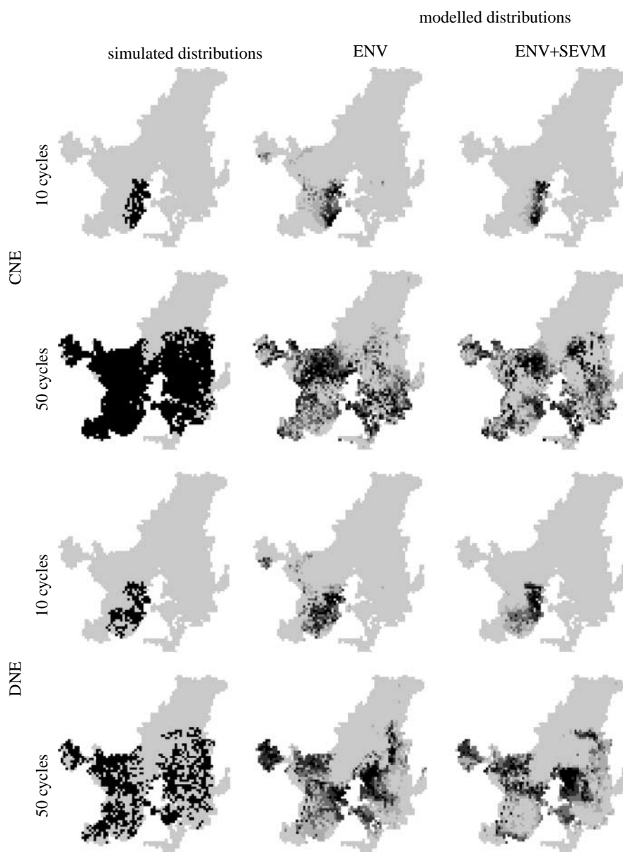
Figure 1. Simulated range distribution under two scenarios of non-equilibrium (CNE and DNE) at two selected time steps and their predicted distribution obtained by modelling environment alone (ENV) or environment coupled with spatial eigenvectors (ENV+SEVM).
