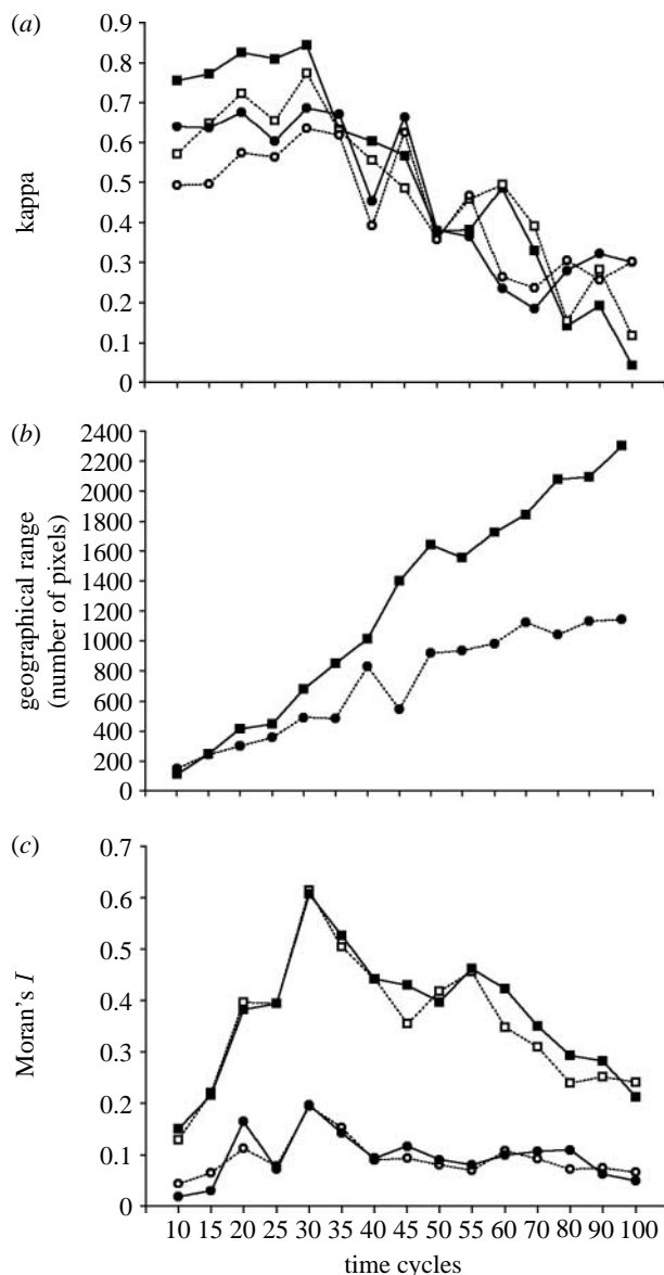
Figure 2. (a) Kappa statistics (open squares, CNE-ENV; filled squares, CNE-ENV-SEVM; open circles, DNE-ENV; filled circles, DNE-ENV-SEVM), (b) range size (squares, CNE; circles, DNE) and (c) residual autocorrelation (Moran's I ) in the first distance class for MAXENT based on environment and spatial eigenvectors models under CNE and DNE simulations across time cycles (open squares, CNE-ENV; filled squares, CNE-ENV-SEVM; open circles, DNE-ENV; filled circles, DNE-ENV-SEVM).
